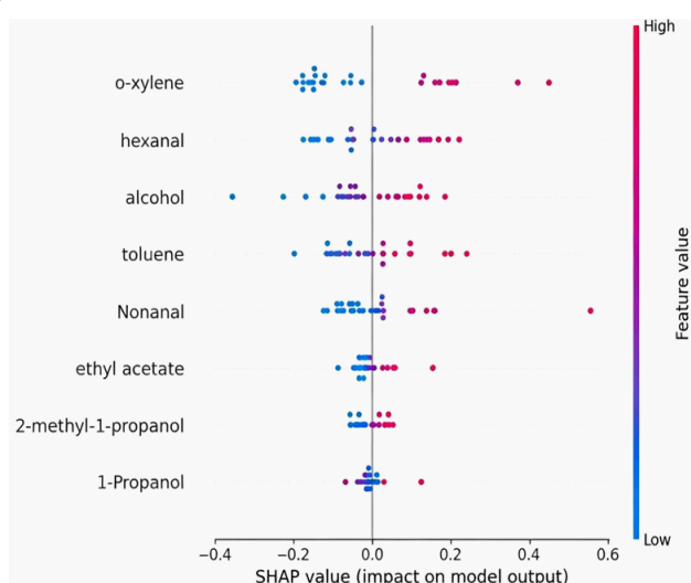
Figure 14: Beeswarm plot of SHAP values for the selected optimal features.
