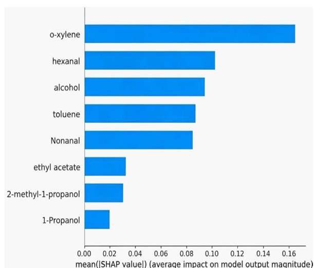
Figure 13: Histogram of feature importance for the selected optimal features, sorted by SHAP value.
